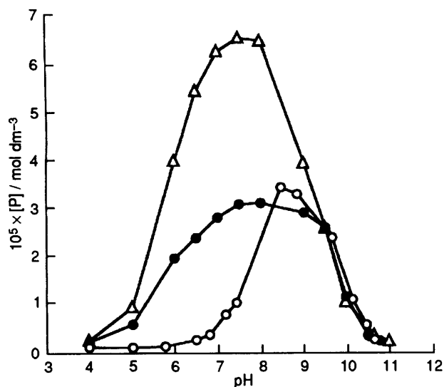
Fig. 2 Plots of [ p -nitroaniline (P)] vs. pH: 37 °C, [ \alpha -chymotrypsin] = 6.08 \times 10^{-7} mol dm -3 , [Sub] = 7.56 \times 10^{-5} mol dm -3 , [phenylboronic acid] = 6.31 \times 10^{-3} mol dm -3 , [saccharide] = 7.69 \times 10^{-2} mol dm -3 : (Δ) control [in the absence of phenylboronic acid and in the presence of D-fructose ( 7.69 \times 10^{-2} mol dm -3 )]; (●) in the presence of phenylboronic acid, and (○) in the presence of phenylboronic acid and D-fructose
